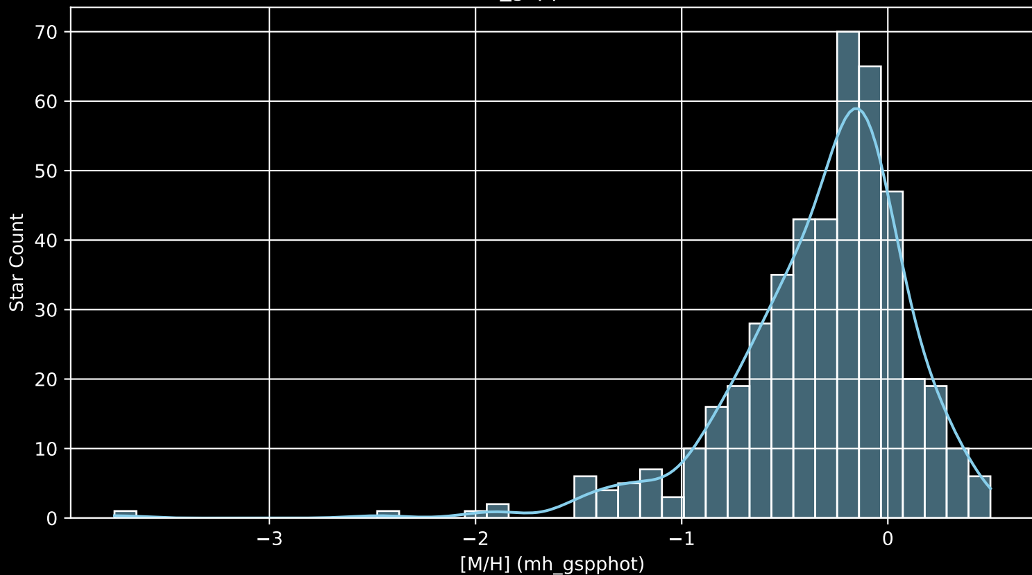
APOGEE DR17 Field: [M3 [M/H] (mh_gspphot) (n= 461)
