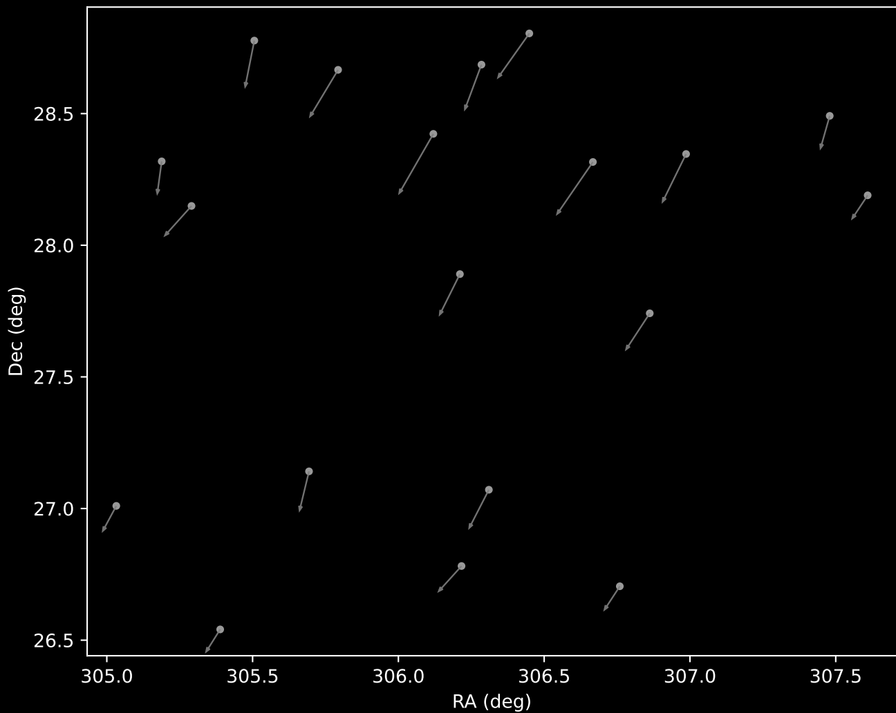
APOGEE DR17 Cluster 14 Proper Motion Vectors (n=19)
