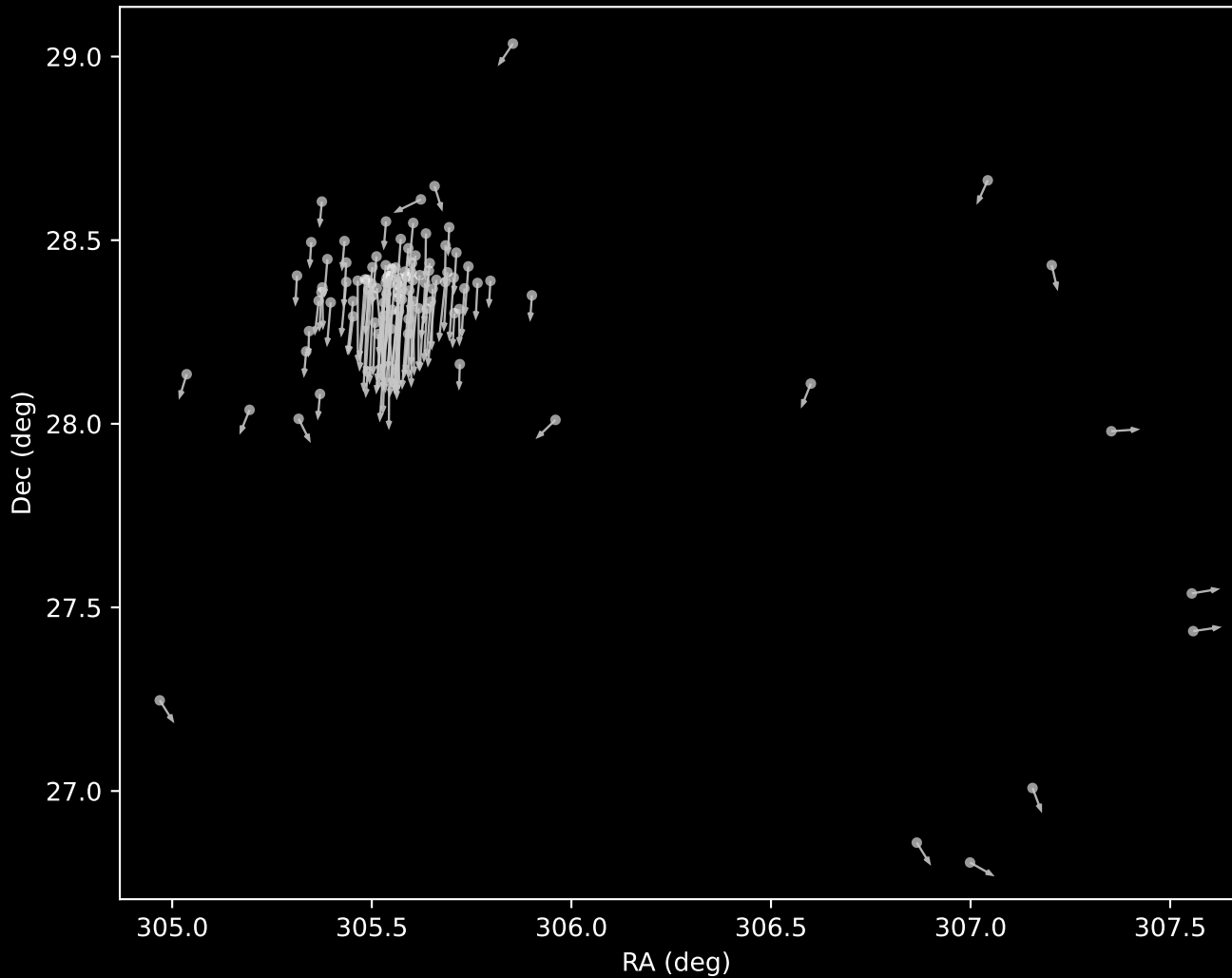
APOGEE DR17 Cluster 15 Proper Motion Vectors (n=103)
