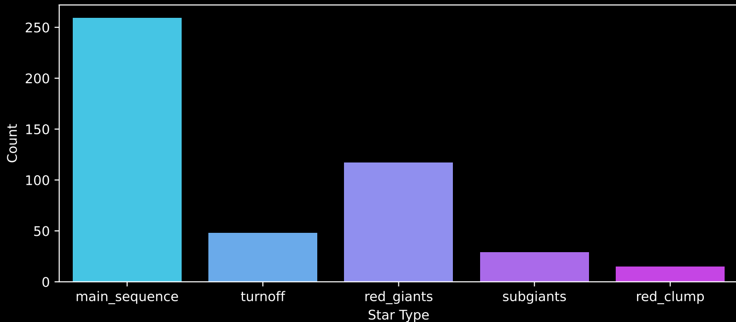
APOGEE DR17 Field: [M3] Count plot of Star Type
