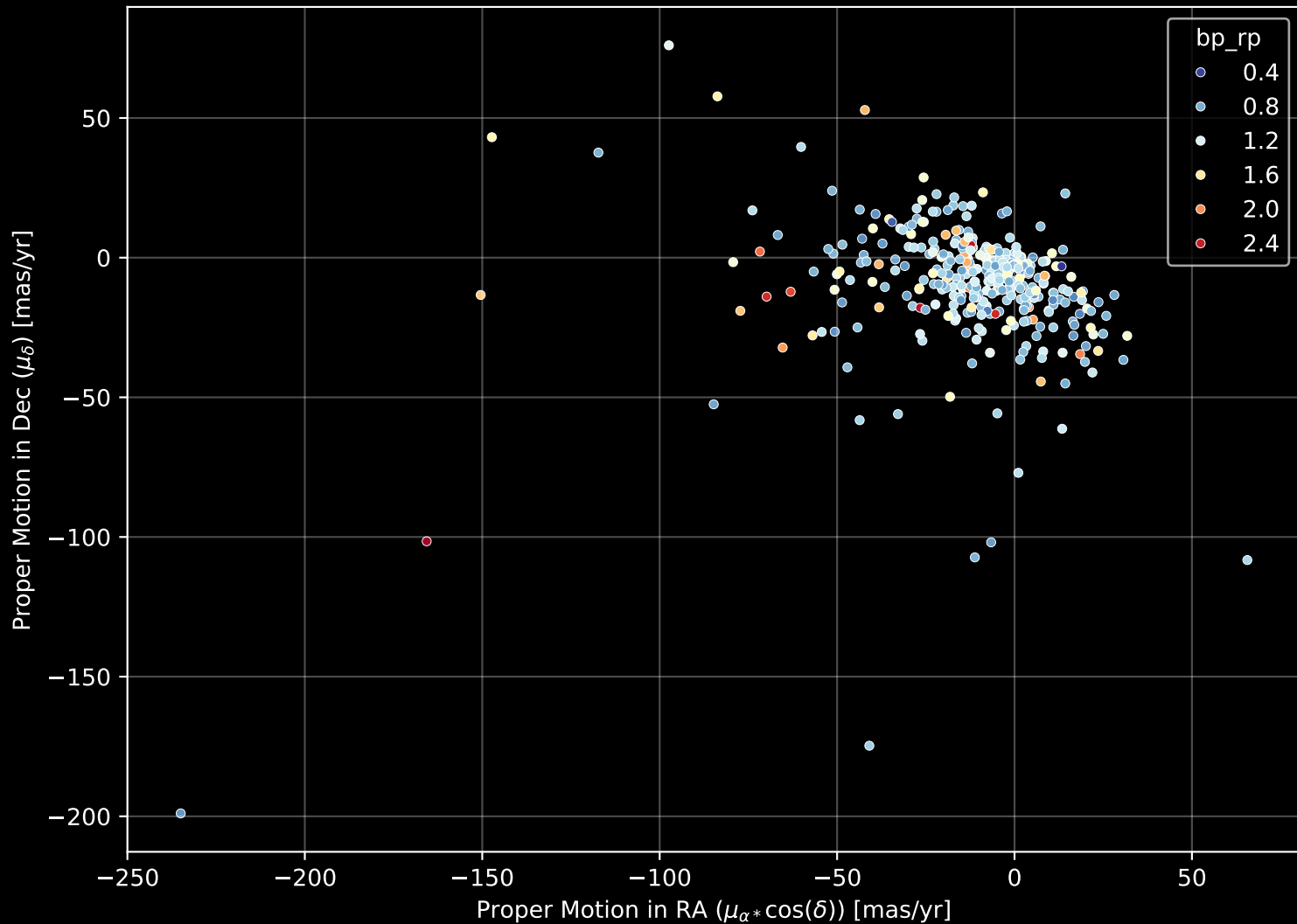
APOGEE DR17 Field: [M3] Proper Motion Diagram (n= 468)
