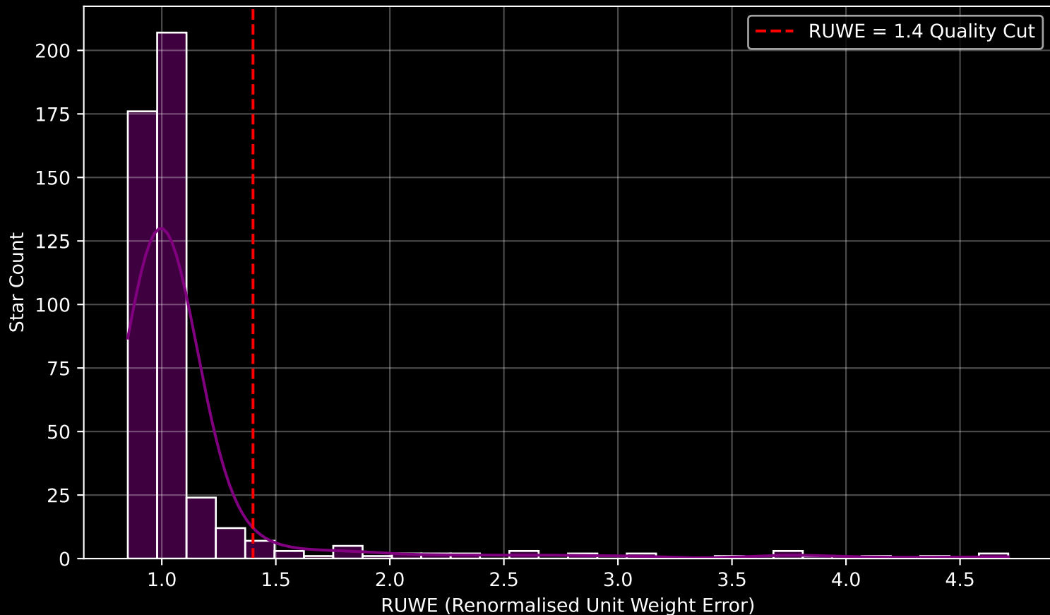
GAPOGEE DR17 Field [M3] RUWE Distribution (n= 458)
