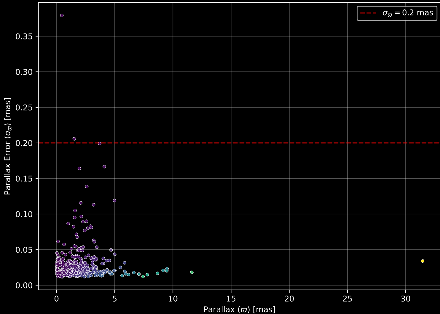
APOGEE DR17 Field: [M3] Parallax Quality (n= 468)
